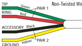
C. Quad Wire*, Solid-Color, Non-Twisted Wire
