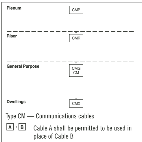
Figure 800-53. Cable Substitution Hierarchy
