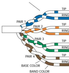
A. Band-Striped Twisted Pair Wire
