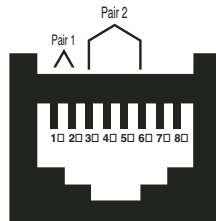
10BASE-T (802.3)
