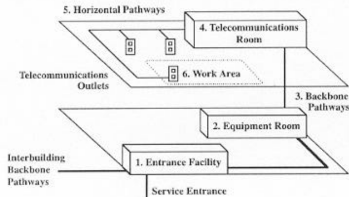
Scope of ANSI/TIA/EIA-569-A
